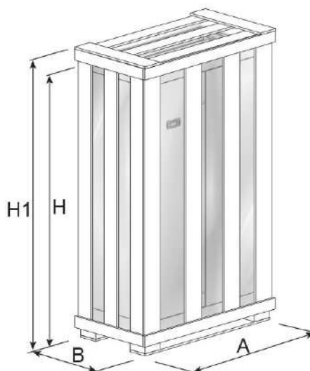
OPTIONAL 9973: WOODEN CAGE PACKING DIMENSIONS
