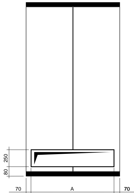
AIR INTAKE FROM THE BACK SIDE
